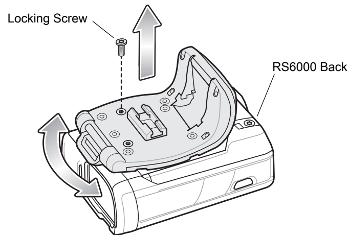
Figure 61 Removal of Trigger Assembly
