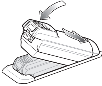
Figure 50 Insert Battery into Slot
