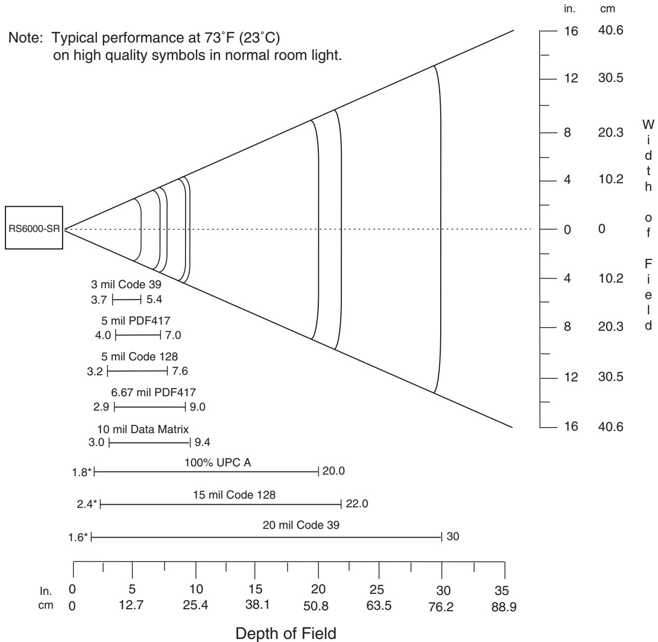
Figure 75 RS6000 Standard Range Decode Zone
