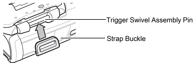
Figure 74 Strap Buckle Installation
