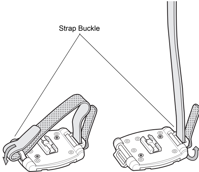
Figure 71 Remove Finger Strap (Triggerless Strap Holder)
