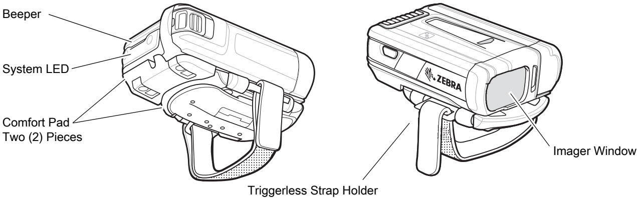
Figure 2 RS6000 Triggerless Configuration Features
