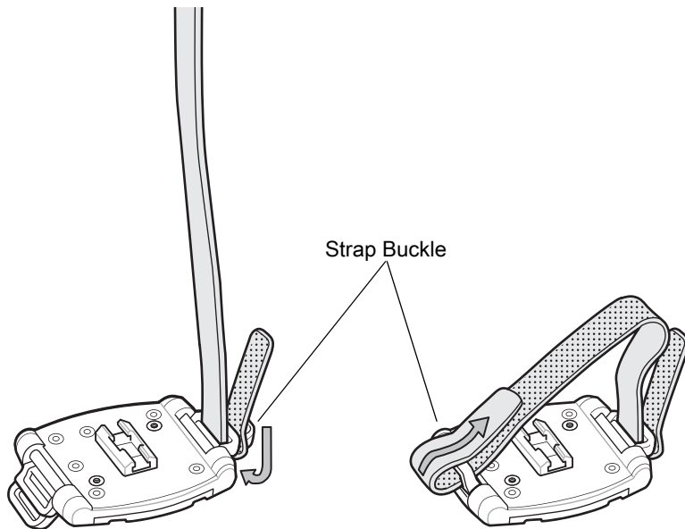
Figure 72 Install Finger Strap (Triggerless Strap Holder)
